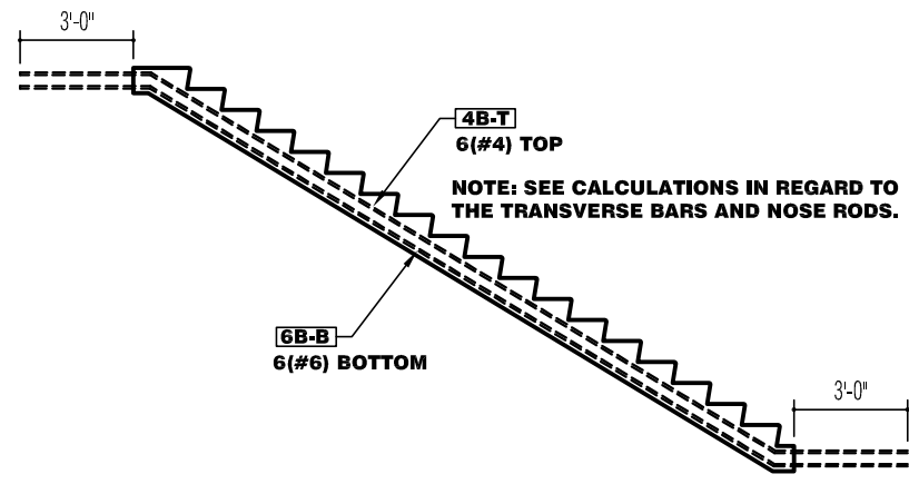
STAIR SECTION w/ REBAR (LEVELS 2-35) 1/4" = 1'-0"
