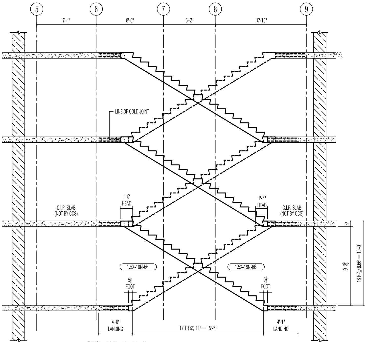
A STAIR #1 & #2 - PLAN (LEVELS 2-35) (STAIR #3 & #4 MIRROR IMAGE) 1/4" = 1'-0"
